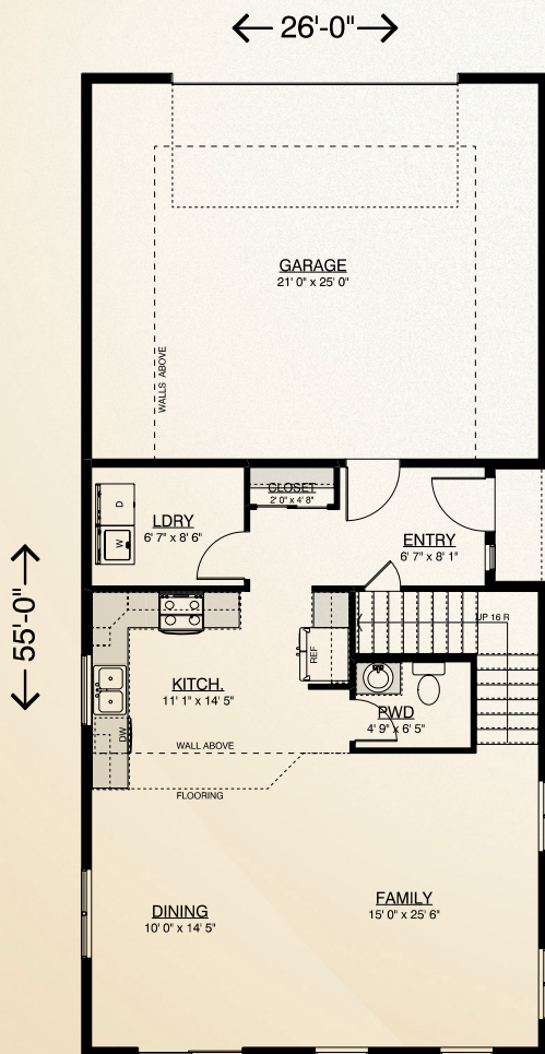
ASH CREEK- MAIN FLOOR
